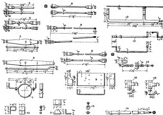
Figs. 2653-2666. Forged Details of Foundation Brake Gear for Tender of Atlantic (1-4-2) Locomotive. P. R. R.
